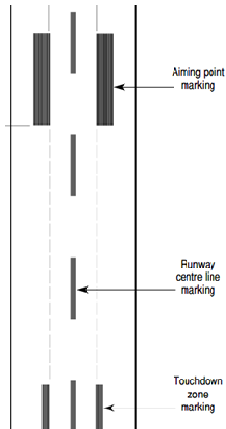
Figure 21 - Touch Down Zone and Aiming Point Markings
