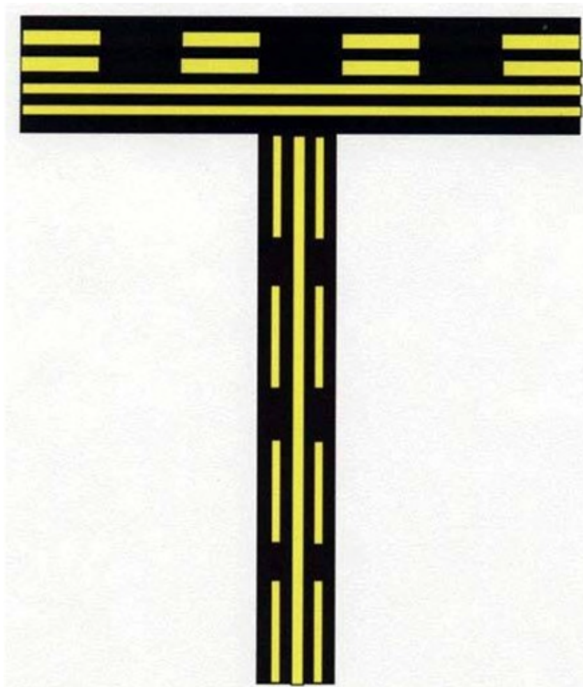
Figure 11 - Enhanced Taxiway Centre Line Attached to Mandatory Hold Position
