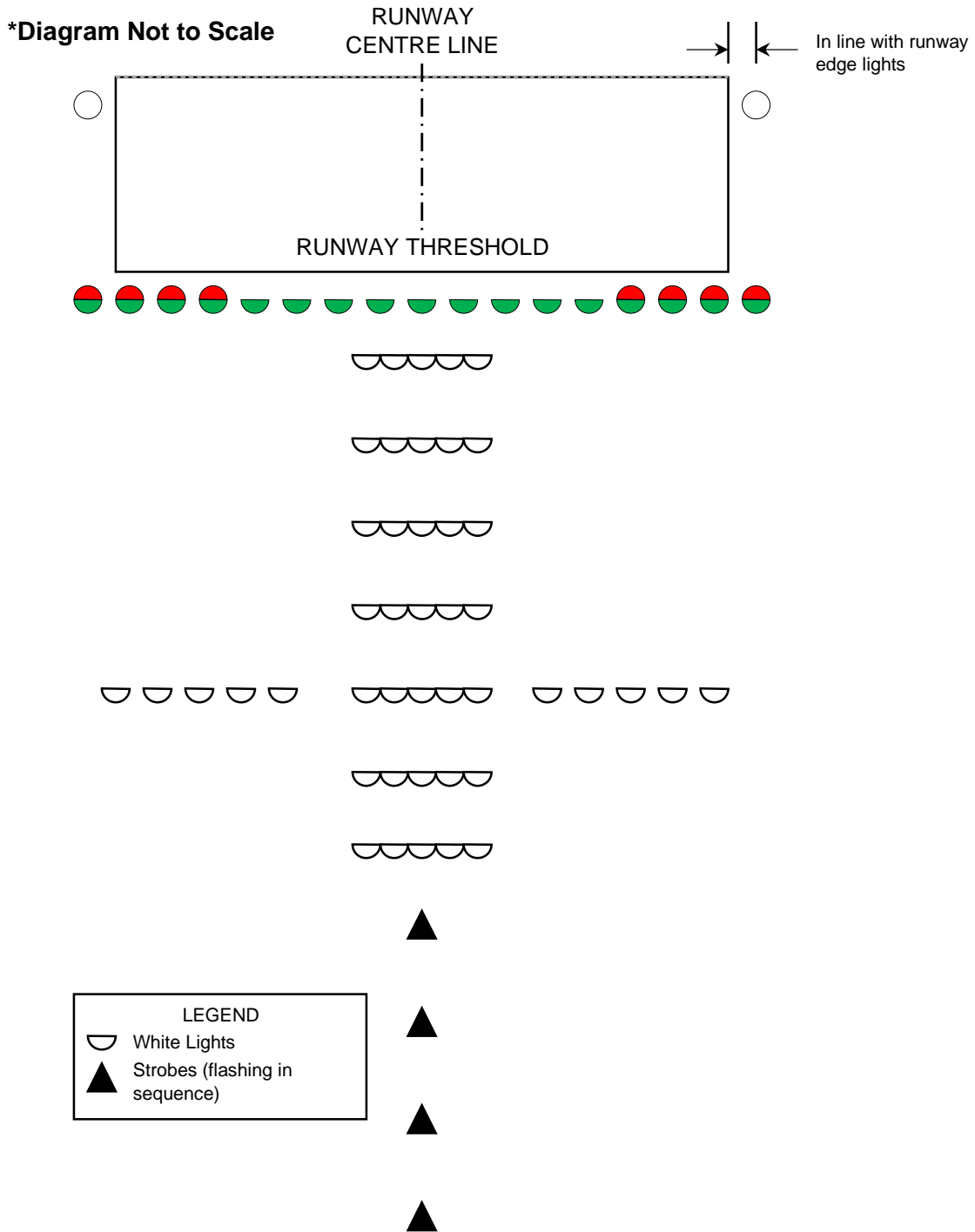
Figure 467 - Short Simplified Approach Lighting with Runway Alignment Indicator Lights (SSALR) Diagram
