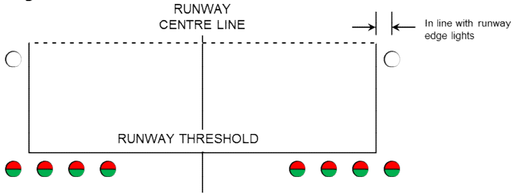
Figure 28 - Runway End and Threshold Lights on Runways 04, 12, and 30 Diagram
