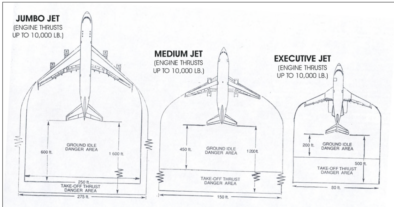
Figure 1 - Jet Blast Danger Areas (Not to Scale)
