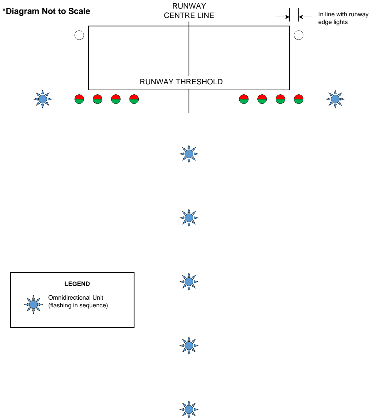
Figure 445 - Omni-Directional Approach Lights (ODALs) Diagram
