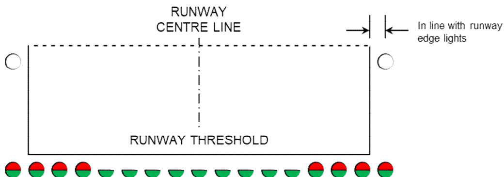
Figure 29 - Runway End and Threshold Lights on Runway 22 Diagram
